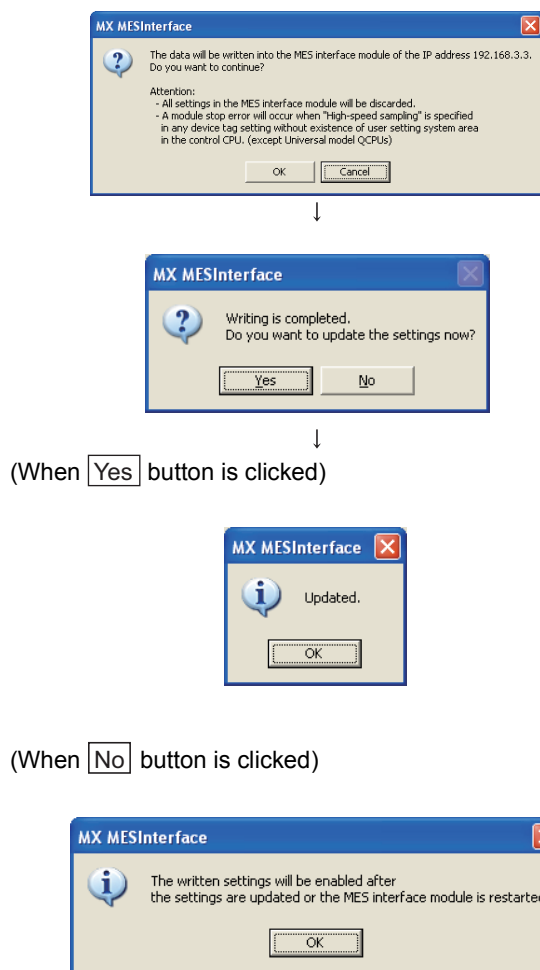
Figure 7.90 Writing the MES interface function settings
