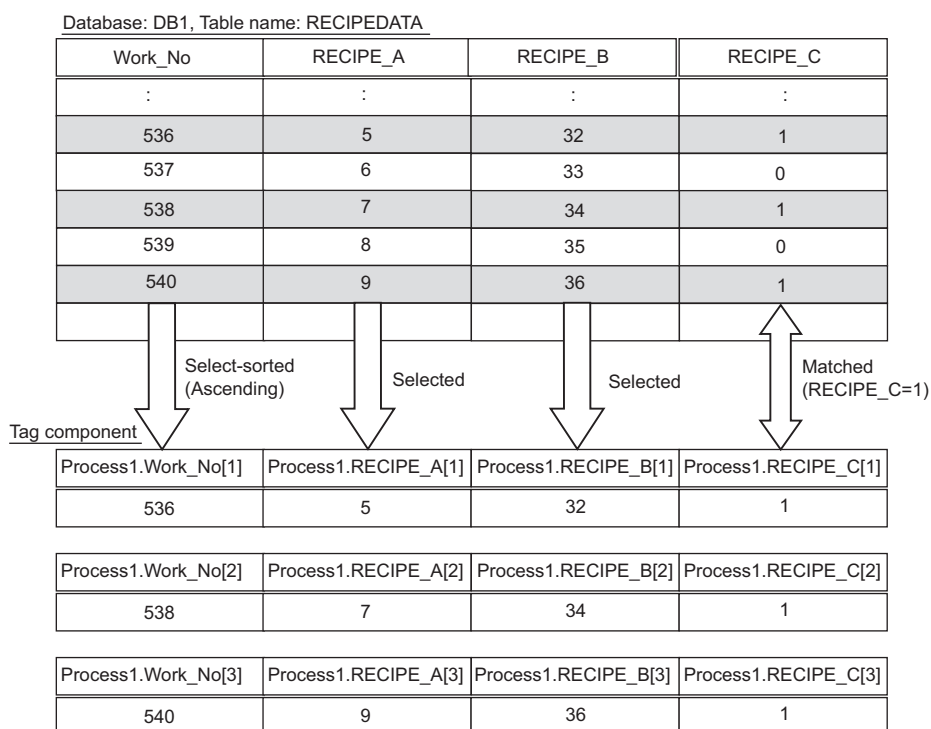
Figure 7.77 An example of [MultiSelect] operation
