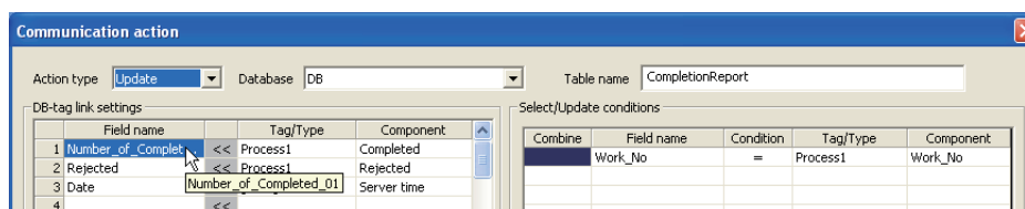
Figure 7.4 Checking with the mouse cursor
