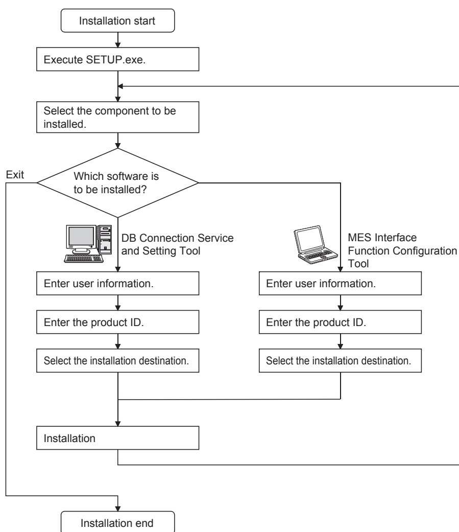
Figure 5.1 MX MESInterface installation procedure
