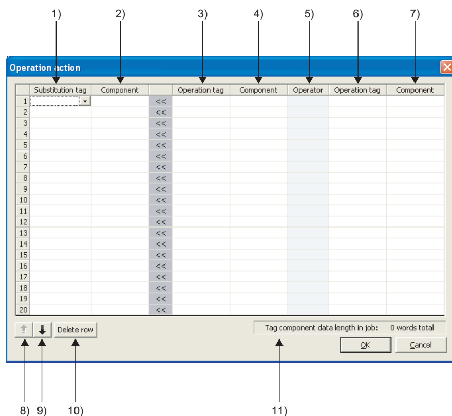
Figure 7.87 [Operation action] dialog box
