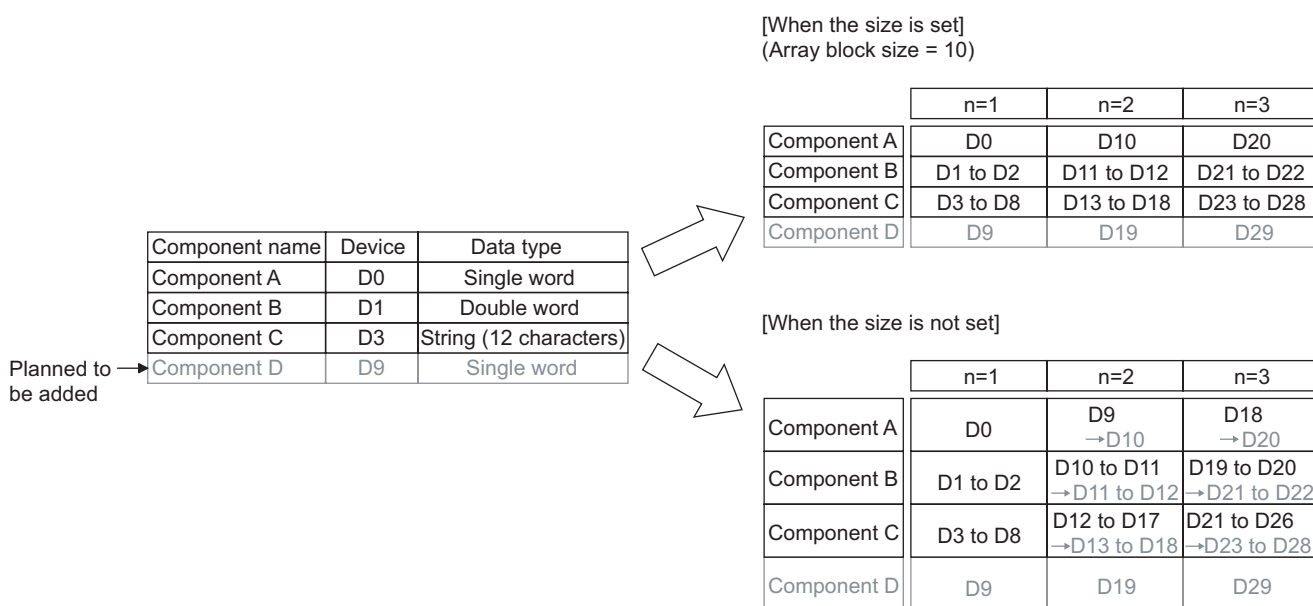
Figure 7.39 An example of [array block size]
