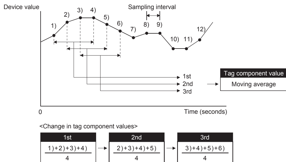
Figure 7.36 Moving average
