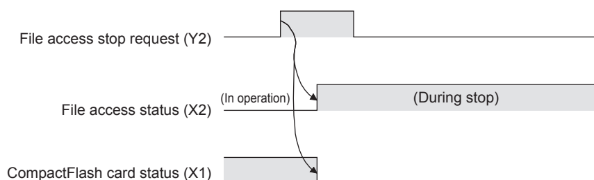
Figure 4.13 File access stop processing
