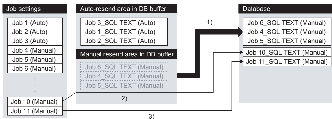
Figure 6.15 Manually resending data
