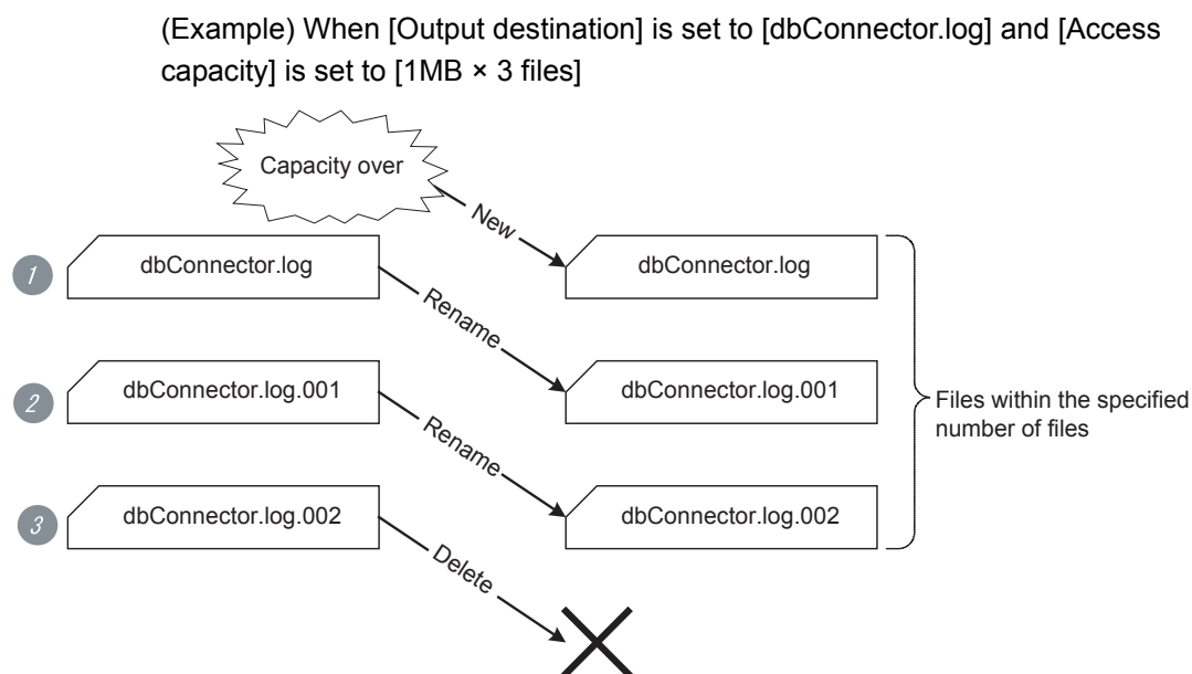
Figure 8.9 File capacity per access log and number of files
