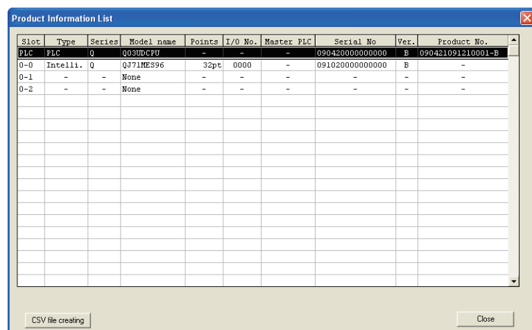
Figure 2.9 [Product Information List] of GX Developer
