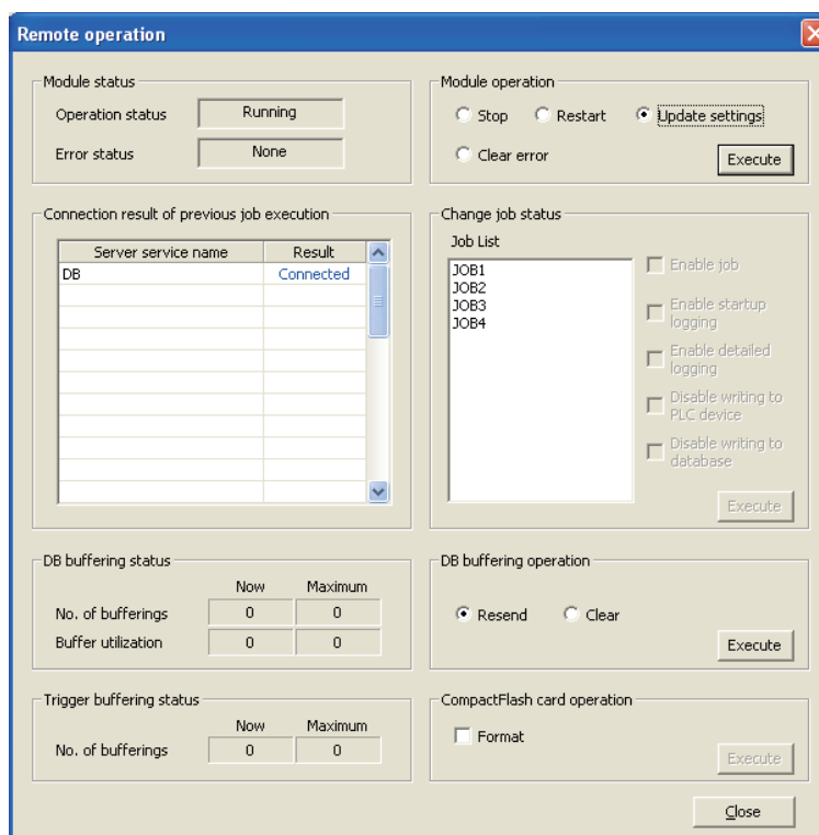
Figure 7.98 [Remote operation] dialog box
