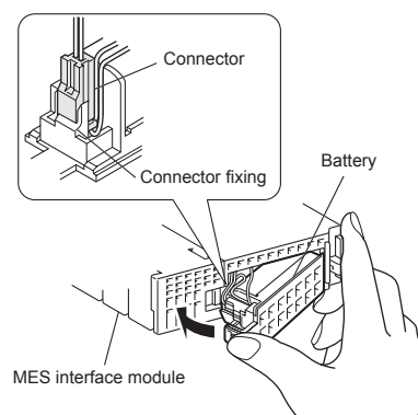
Figure 4.18 Battery mounting procedure
