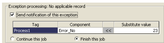
Figure 7.82 Setting example of [Exception processing: No applicable record]
