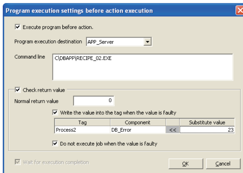
Figure 7.61 [Program execution settings before action execution]
