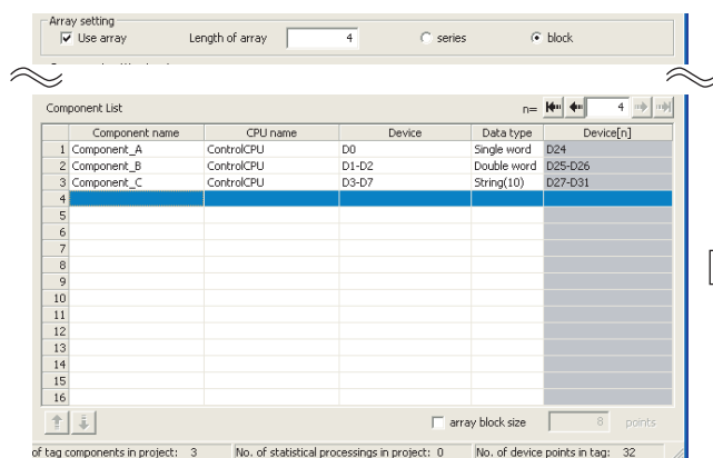
Figure 7.34 When [block] is selected
