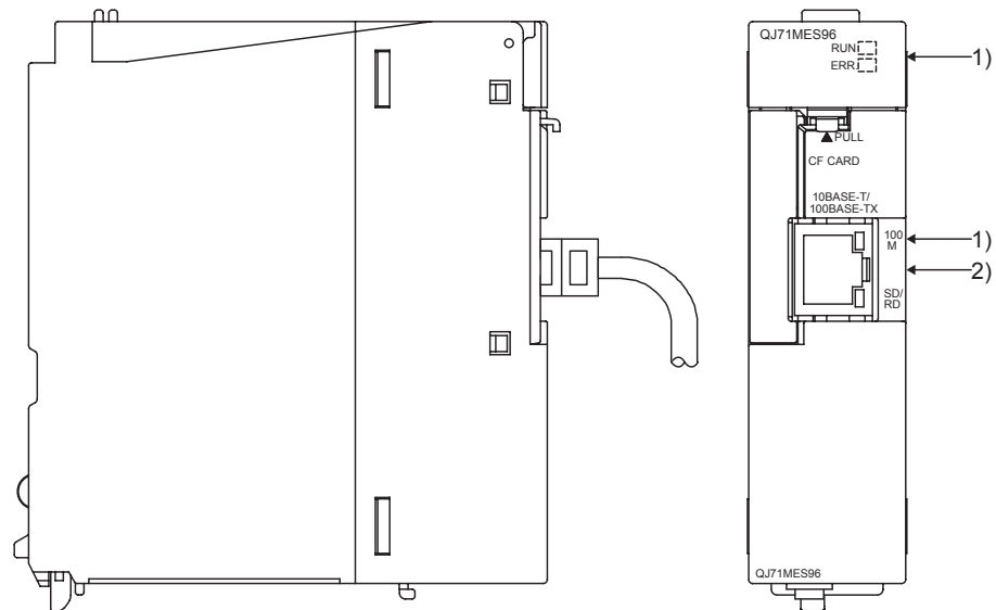
Figure 4.3 With the LED cover closed
