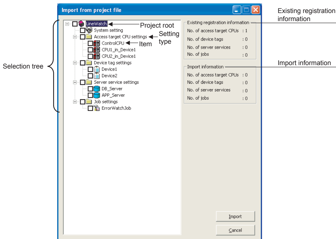
Figure 7.14 [Import from project file] dialog box
