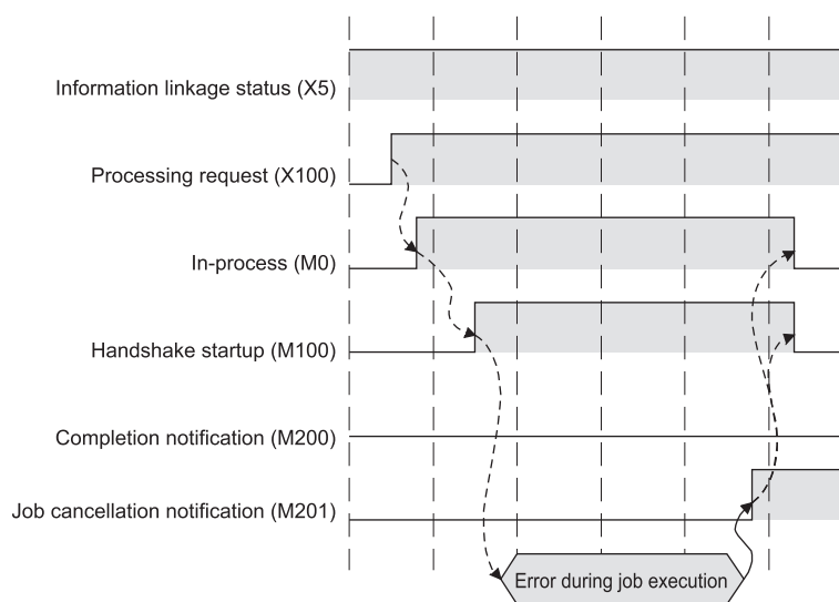
Figure 7.58 When an error occurs during job execution
