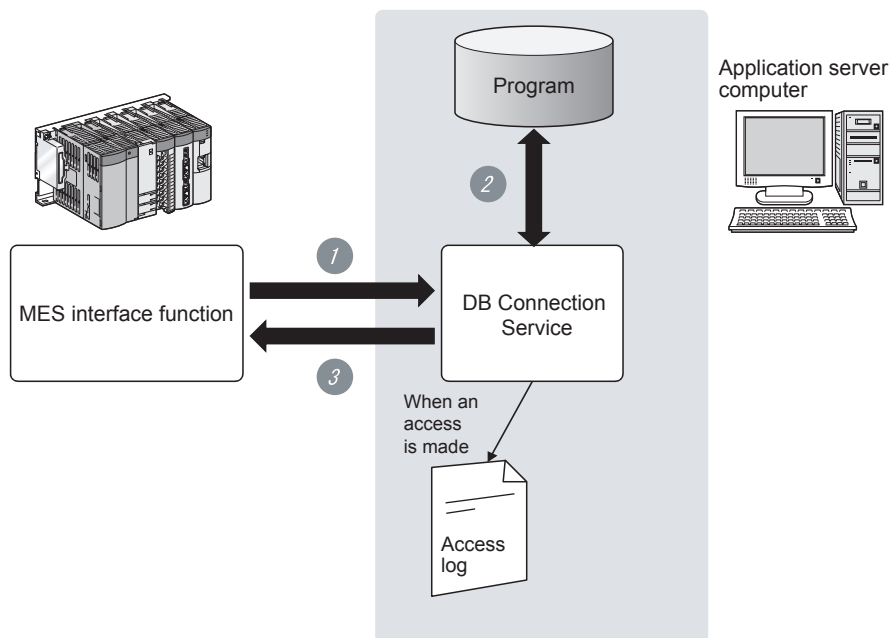
Figure 8.2 Program execution function
