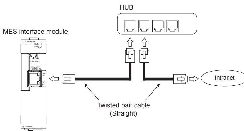
Figure 4.6 Wiring
