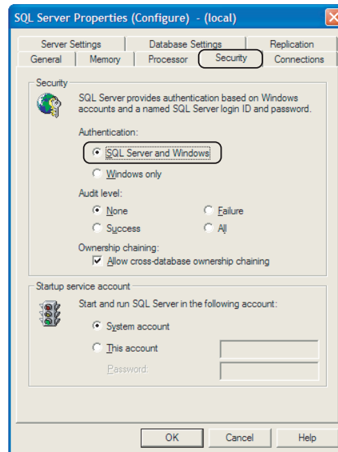
Figure 2.10 [SQL Server Properties (Configure)]
