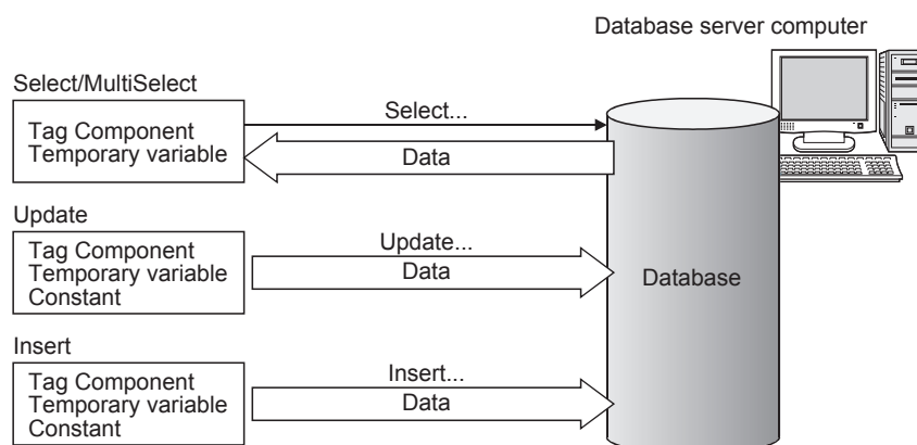
Figure 6.8 SQL text transmission (Communication action)
