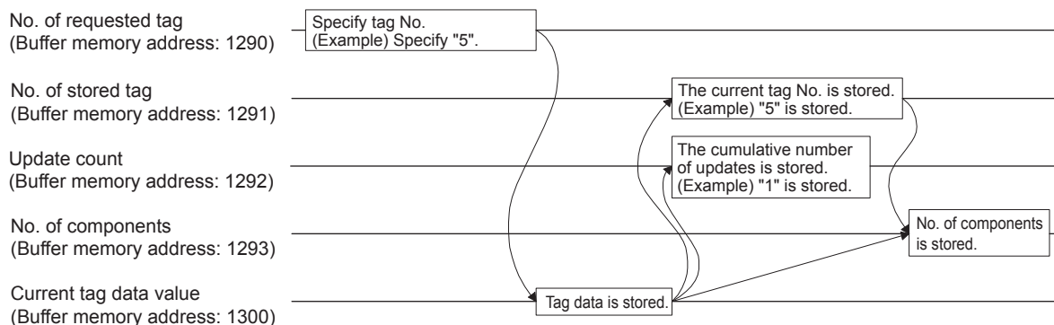
Figure 3.11 Current tag data value area
