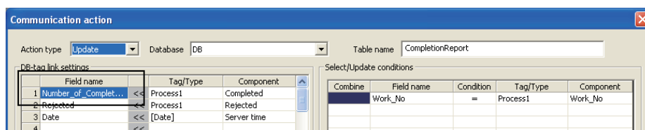
Figure 7.2 Before resizing the column
