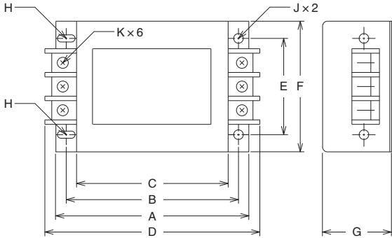
3G3AX-NFO01 3G3AX-NFO02
