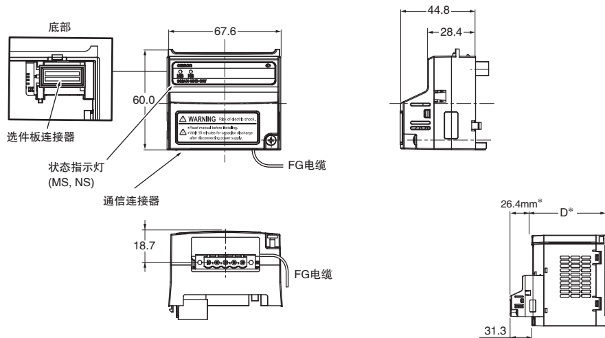
3G3AX-MX2-DRT-E
